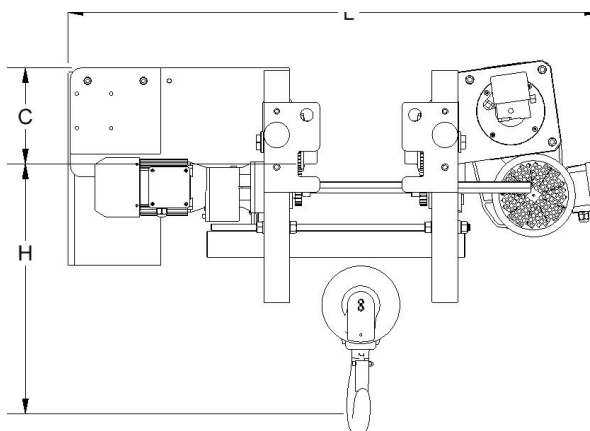
SMW Series Wire Rope Hoist Dimensions
