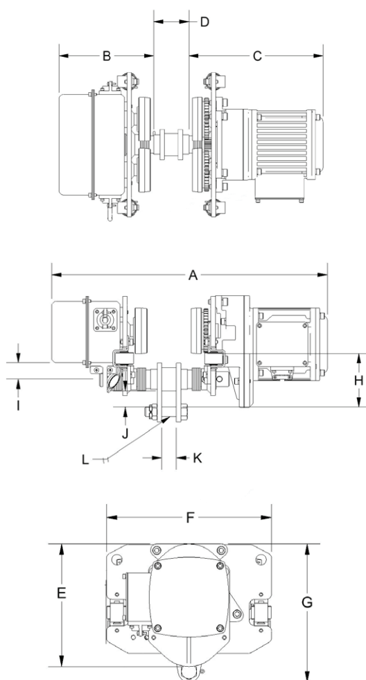
Starke SMT Trolley (Lug Series) Dimensions
